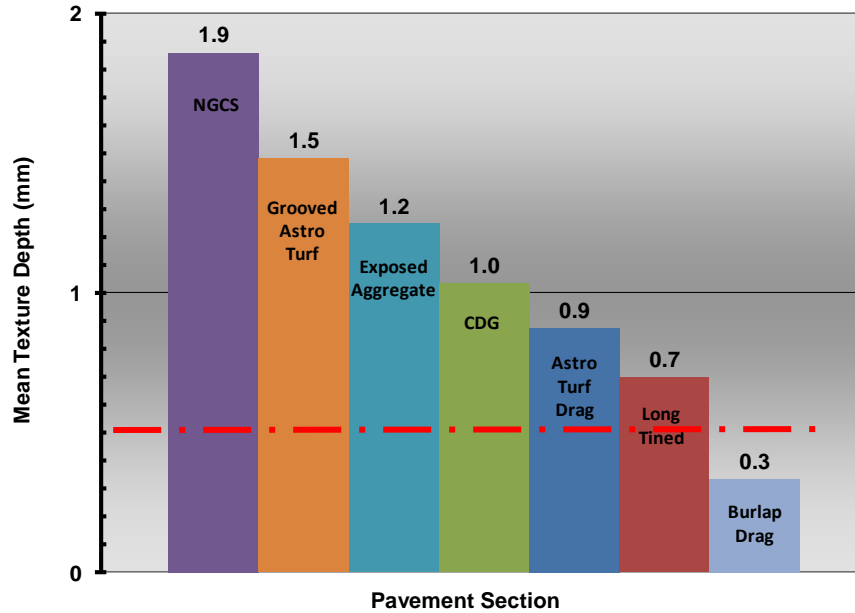
Figure 36 Mean Texture Depths on Kansas I-70 Texture Experiment
