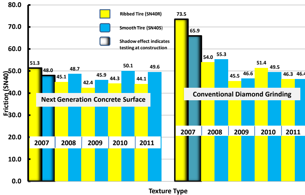
Figure 28 Friction (SN40) as a Function of Surface Texture and Time at MnROAD I-94 WB
