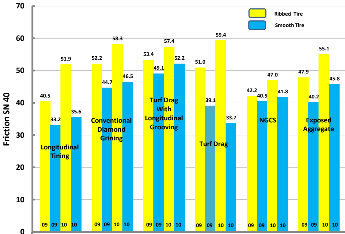
Figure 30 Friction (SN40) as a Function of Surface Texture and Time at KDOT I-70 EB Test Sections
