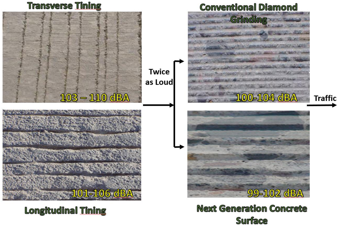
Figure 37 Typical OBSI Levels Measured on Each of the Pavement Textures
