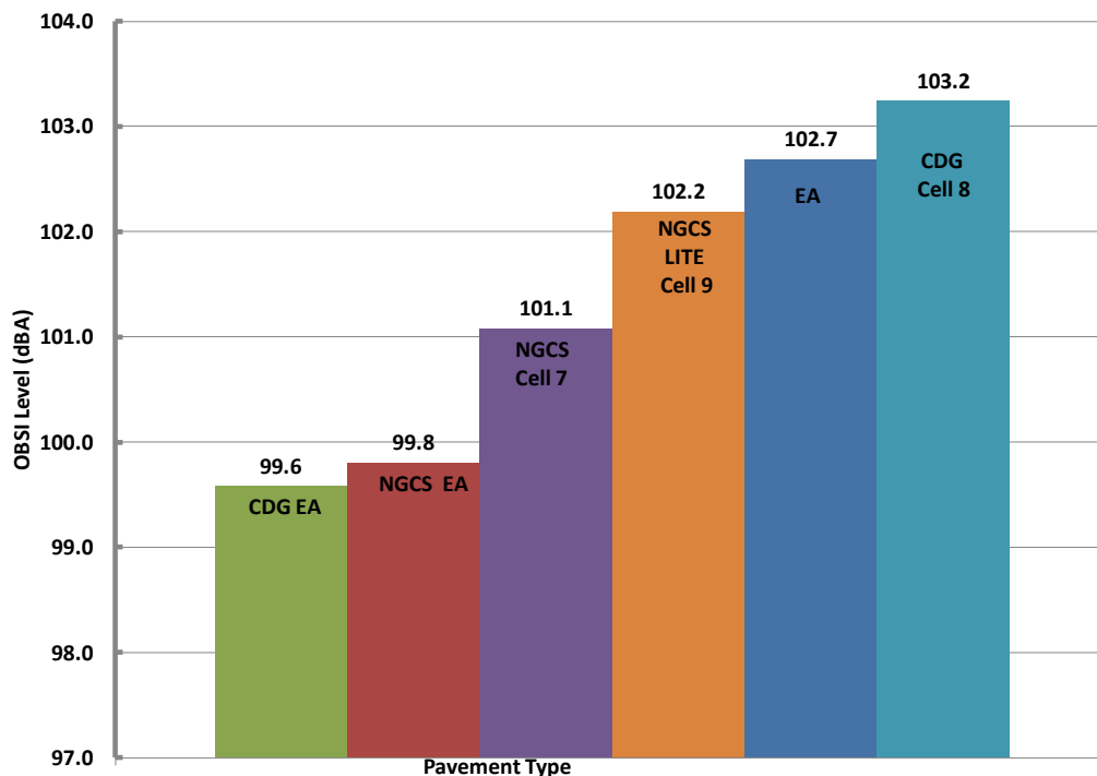
Figure 22 Comparison of Several MnROAD Test Sections to NGCS Test Sections in 2011
