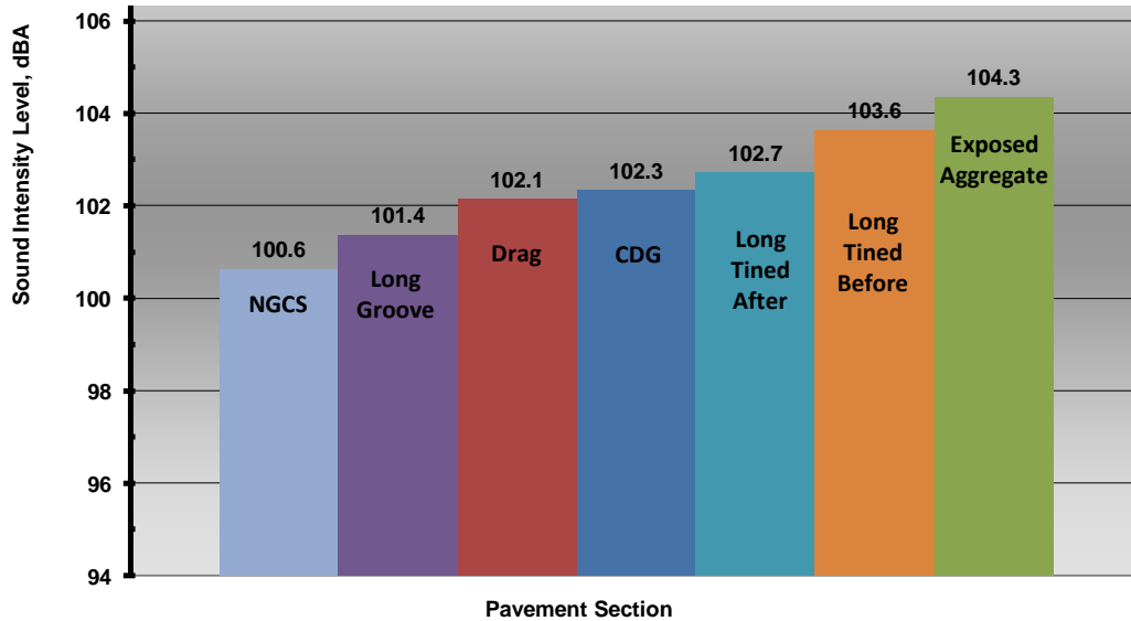
Figure 19 Kansas I-70 EB Surface Texture Test Sections Compared to NGCS in 2011 (3 yrs old)
