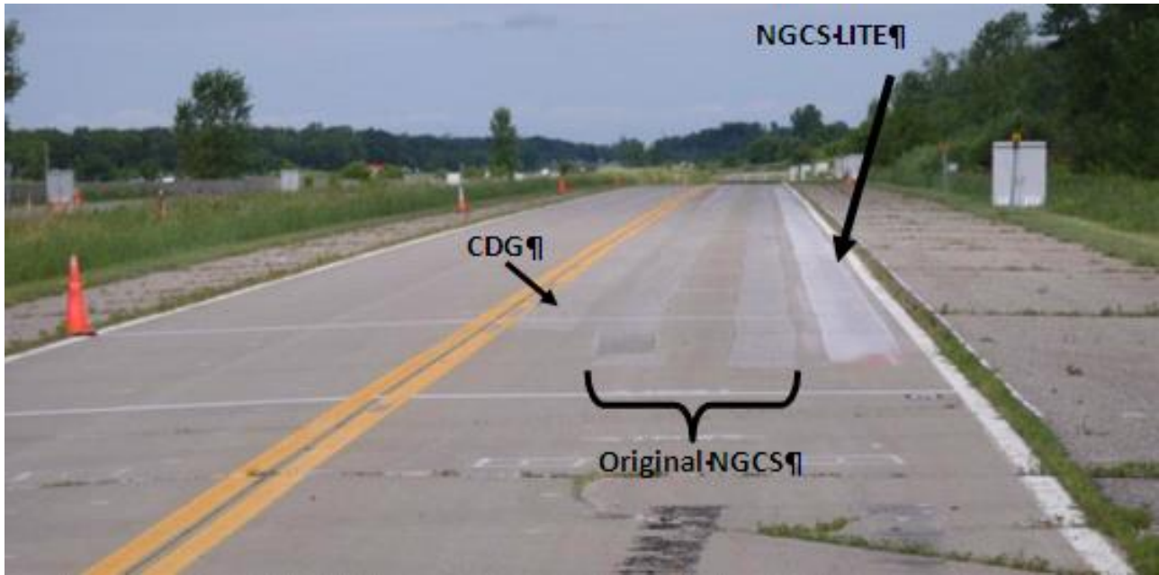
Figure 23 NGCS LITE Test Strip on Cell 37 at MnROAD 13
