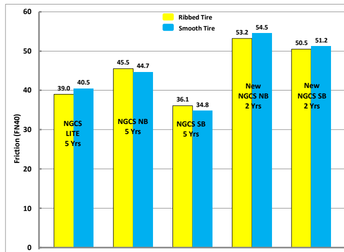
Figure 29 2015 IGGA E274 Friction Results for Duluth Minnesota
