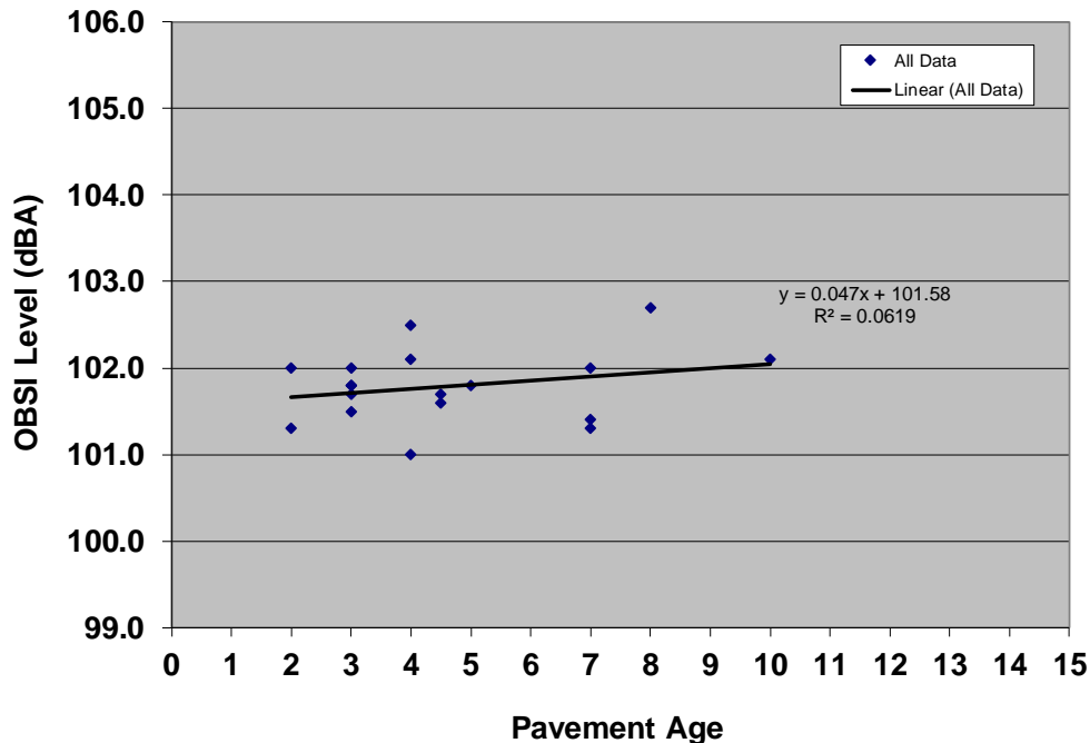
Figure 21 Acoustic Durability of Kansas Diamond Ground Textures (ref 28)
