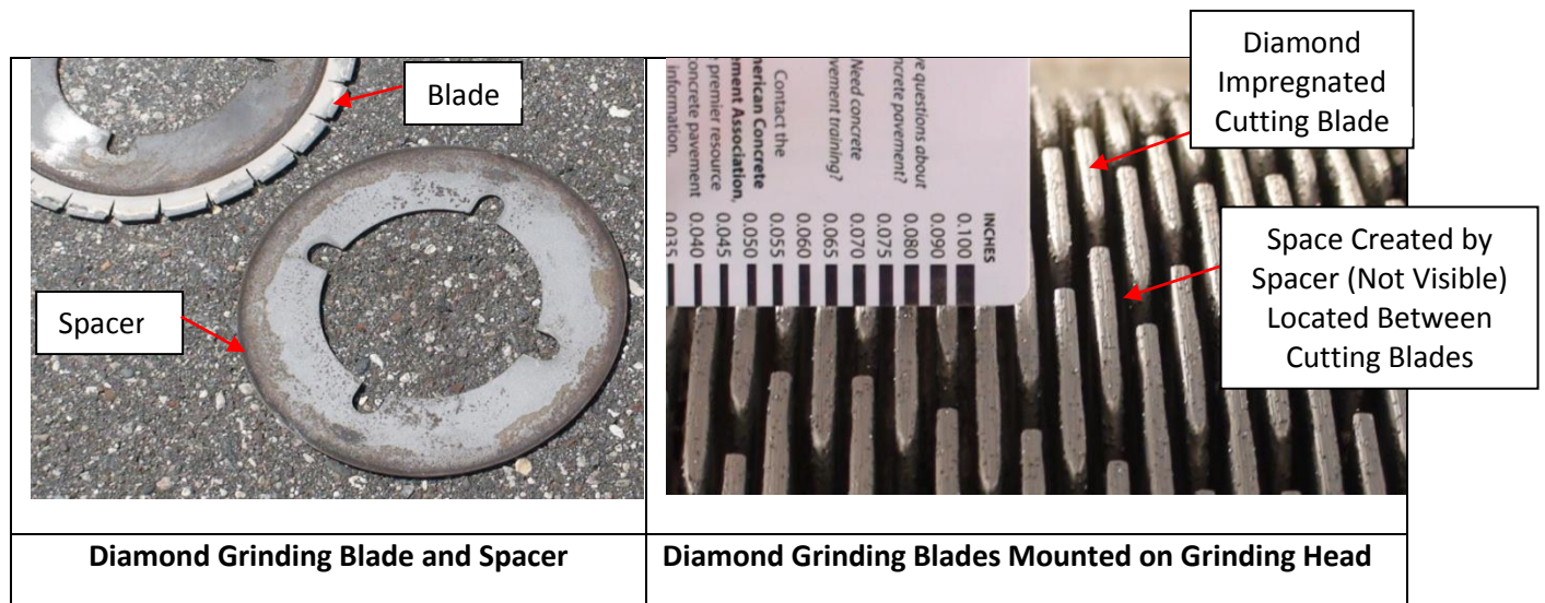
Figure 3 Diamond Impregnated Blades Separated by Spacers (not visible) on Conventional Diamond Grinding Head
