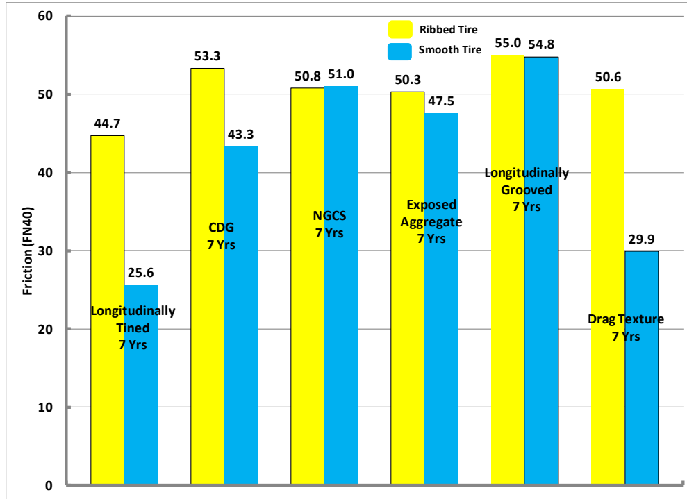
Figure 31 Kansas I-70 IGGA E274 2015 Friction Testing
