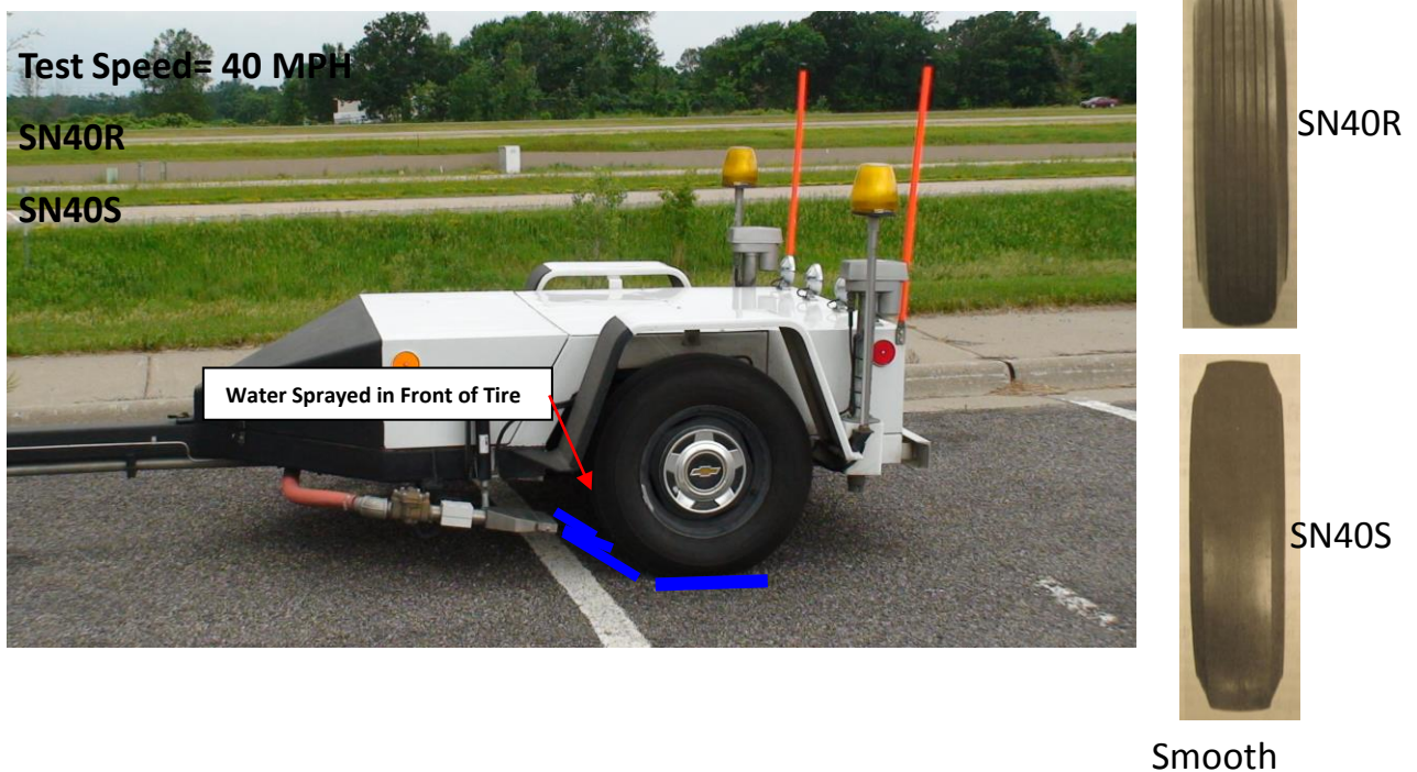
Figure 27 MnDOT ASTM E274 Skid Trailer with ASTM Smooth and Ribbed Tires
