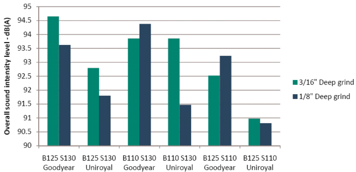
Figure 5 Effect of Grind Depth on OBSI Level 2
