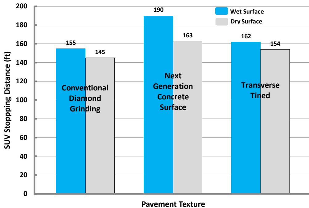
Figure 33 SUV ABS Brake Stopping Distance Testing at Chicago I-355
