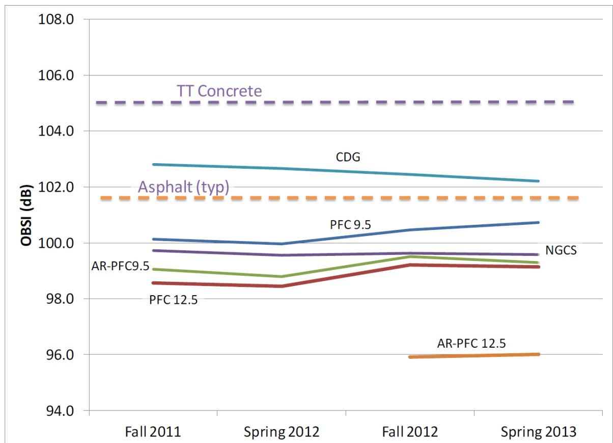
Figure 26 VDOT Quiet Pavement Noise Level Results 30
