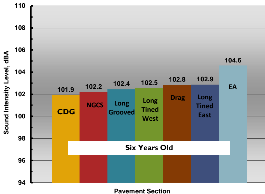
Figure 20 Kansas I-70 2014 OBSI Test Results (dBA)
