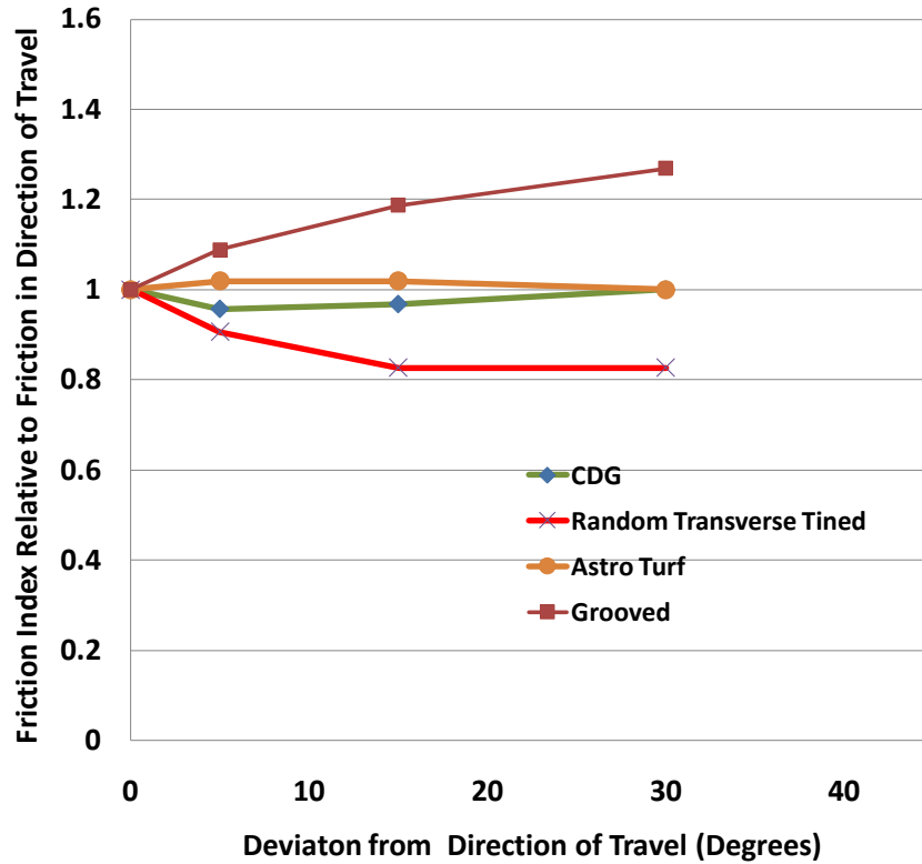
Figure 35 Anisotropic Friction Behavior On Various Concrete Surfaces
